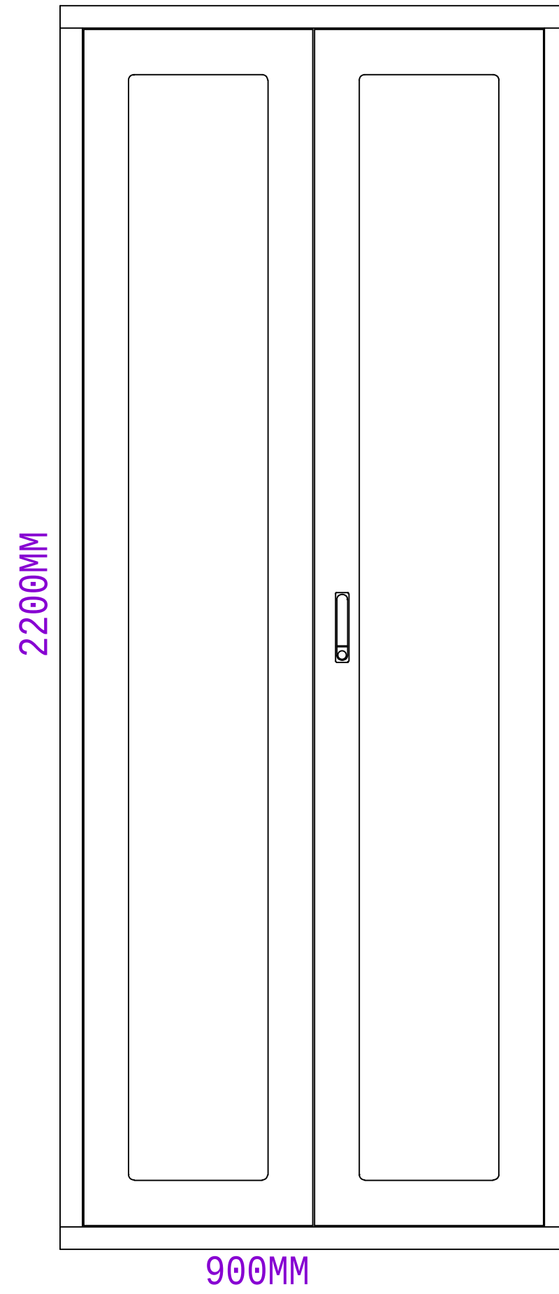
FRONT VIEW
